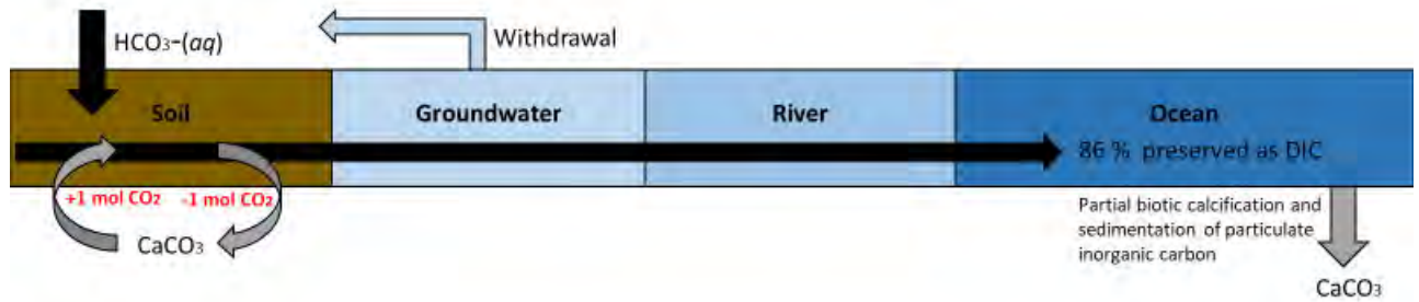
Figure 11: Schematic pathway of \text{HCO}_3^-(\text{aq}) from field to ocean. Considering soil solution, ground- and river water chemistry, substantial precipitation of persistent calcium carbonate is neglectable.
