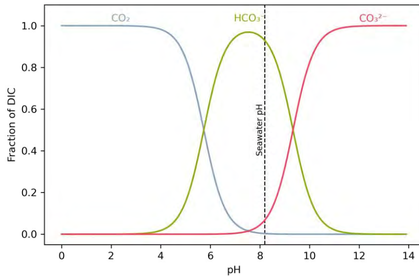
Figure 10: The pH dependent equilibria of dissolved inorganic carbon species. Considering common pH ranges of ground- river or ocean water, the largest share of dissolved inorganic carbon will be present as bicarbonate. Bicarbonate can no longer directly exchange with the atmosphere.
