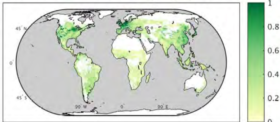
Figure 5: Global overview of NPP norm of annual cropping systems (Source Fig. 6: Modified from Beerling et al. 2020).
